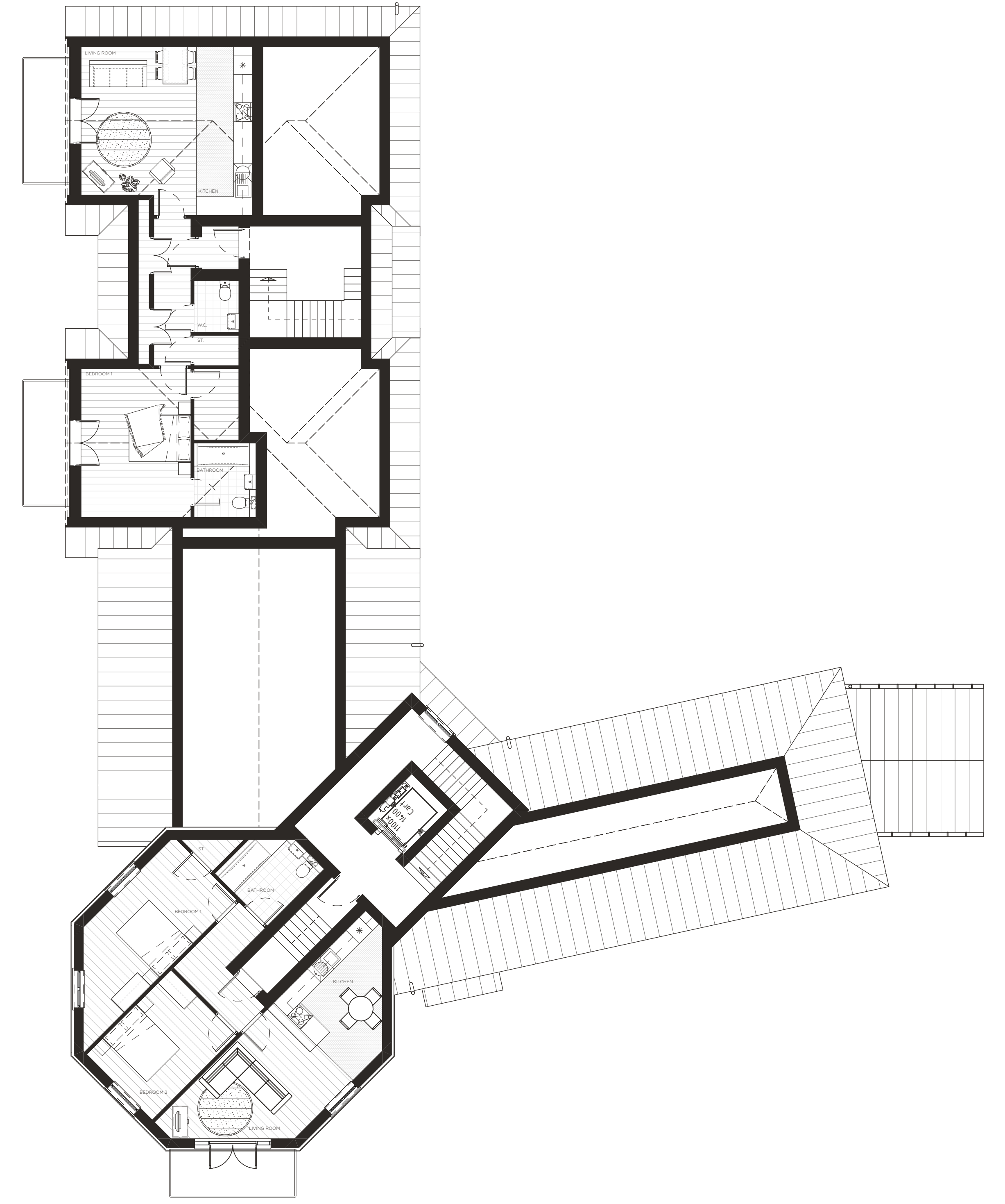
SECOND FLOOR
