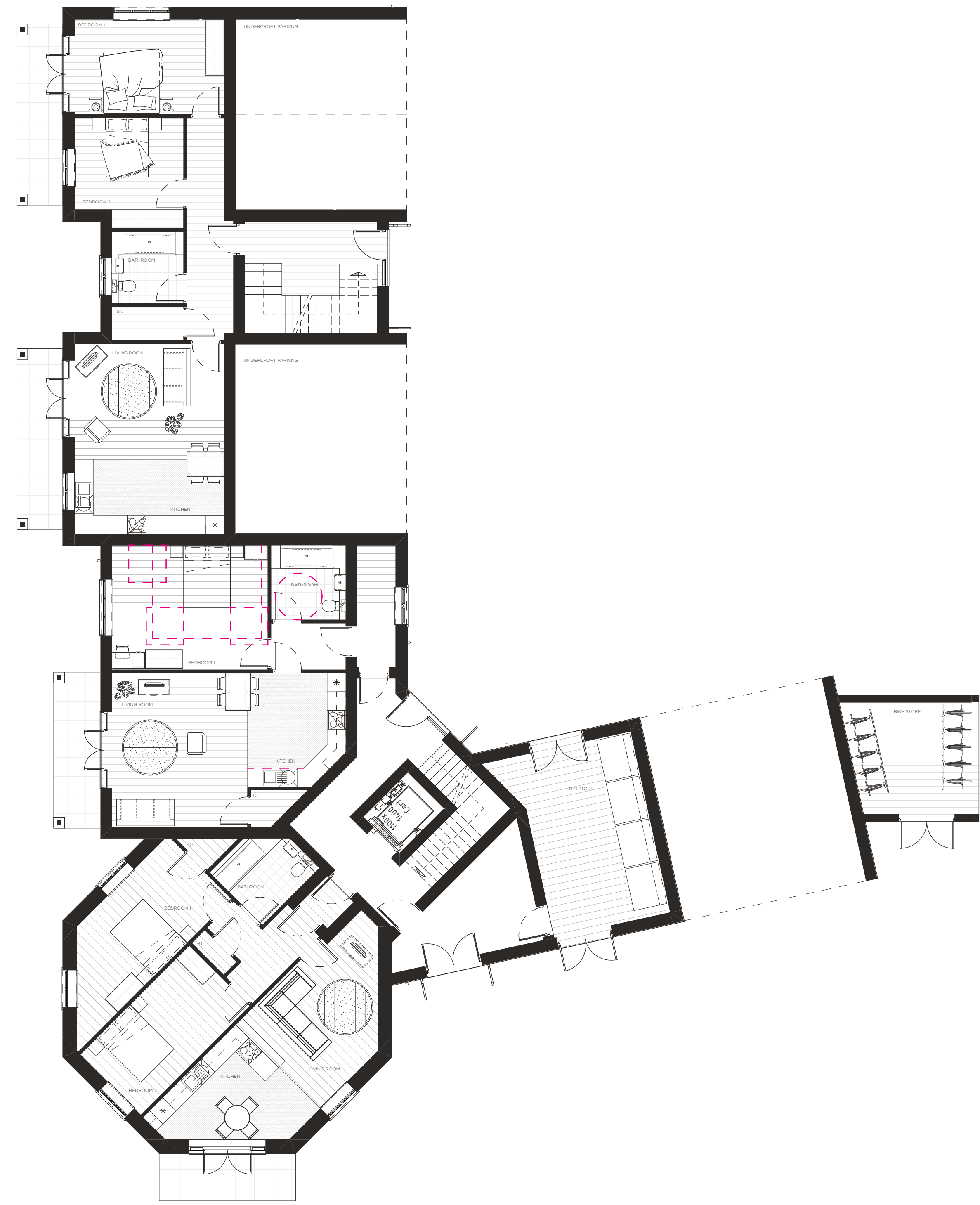
GROUND FLOOR
